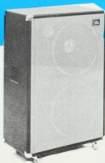
SB.230 Two D.130F in an enclosure incorporating two tuned ports. BB 240 extra heavy duty version with two D.140F speaker 160 watts R.M.S. maximum 94 x 63 x 35
